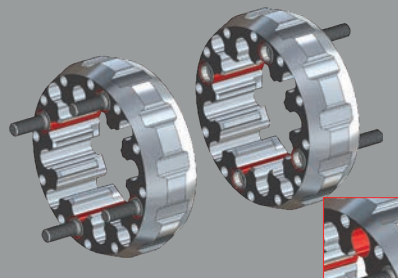
PERFIL I SPECIAL HOLES FOR M12 BOLTS
